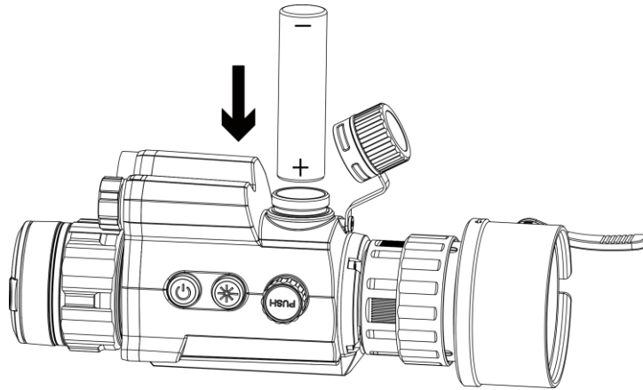
Figure 2-4 Install Battery
