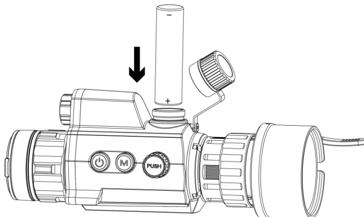
Figure 2-4 Install Battery
