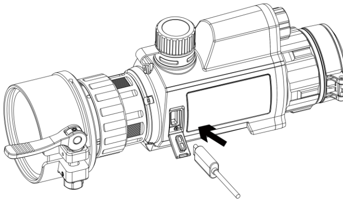
Figure 2-1 Cable Connection
