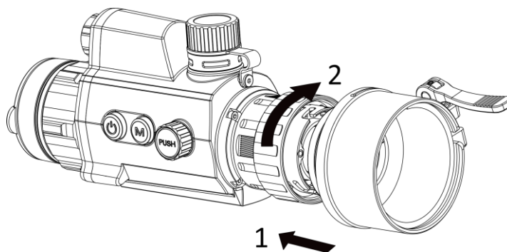
Figure 2-2 Install Adapter
