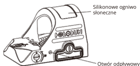
Ryc. 1 Kolimator HS407C X2
