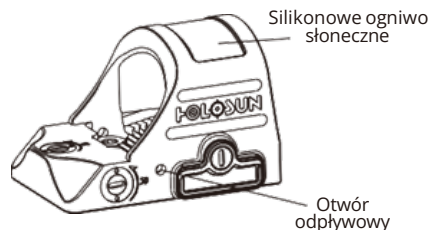
Ryc. 1 Kolimator HE507C-GR X2
